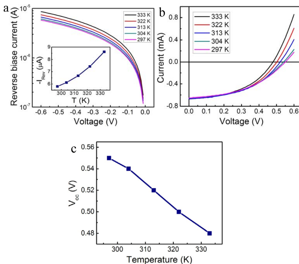
Figure S7: (a) Dark and light (b) I - V curves of the solar cell obtained at 5 different temperatures from 297K to 333K. (c) Open circuit voltage ( V_{\text{oc}} ) decreases with temperature.
