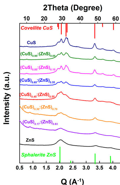
Figure 3. WAXS patterns of (CuS) x :(ZnS) 1- x film at different Cu concentrations, from x = 0 to x = 1 . The expected peak positions of covellite CuS and sphalerite ZnS are indicated by lines at the top and bottom of the plot, respectively.
