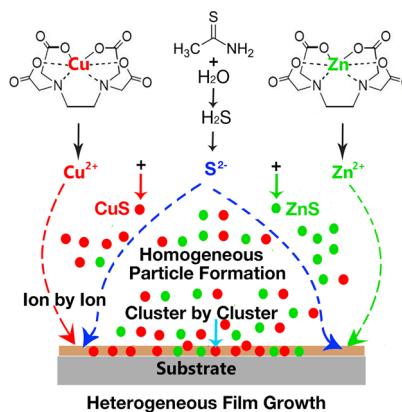
Figure 1. Schematic illustration of the growth mechanism of (CuS) x :(ZnS) 1− x films via chemical bath deposition. Homogeneous nucleation of CuS and ZnS nanoparticles is represented by red and green dots, respectively. This process leads to cluster film growth (cyan arrow). The ion by ion growth process is represented by the dashed red and green arrows.
