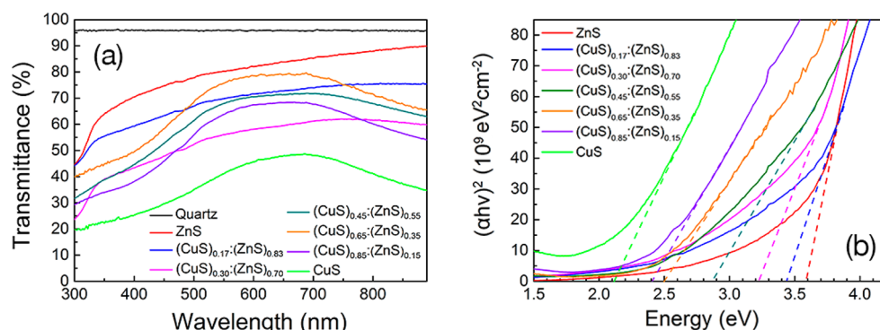
Figure 4. (a) Transmission spectra of (\text{CuS})_x:(\text{ZnS})_{1-x} film (thickness \sim 50 nm) and (b) Tauc plot of (\text{CuS})_x:(\text{ZnS})_{1-x} at different Cu concentrations, from x = 0 to x = 1 .
