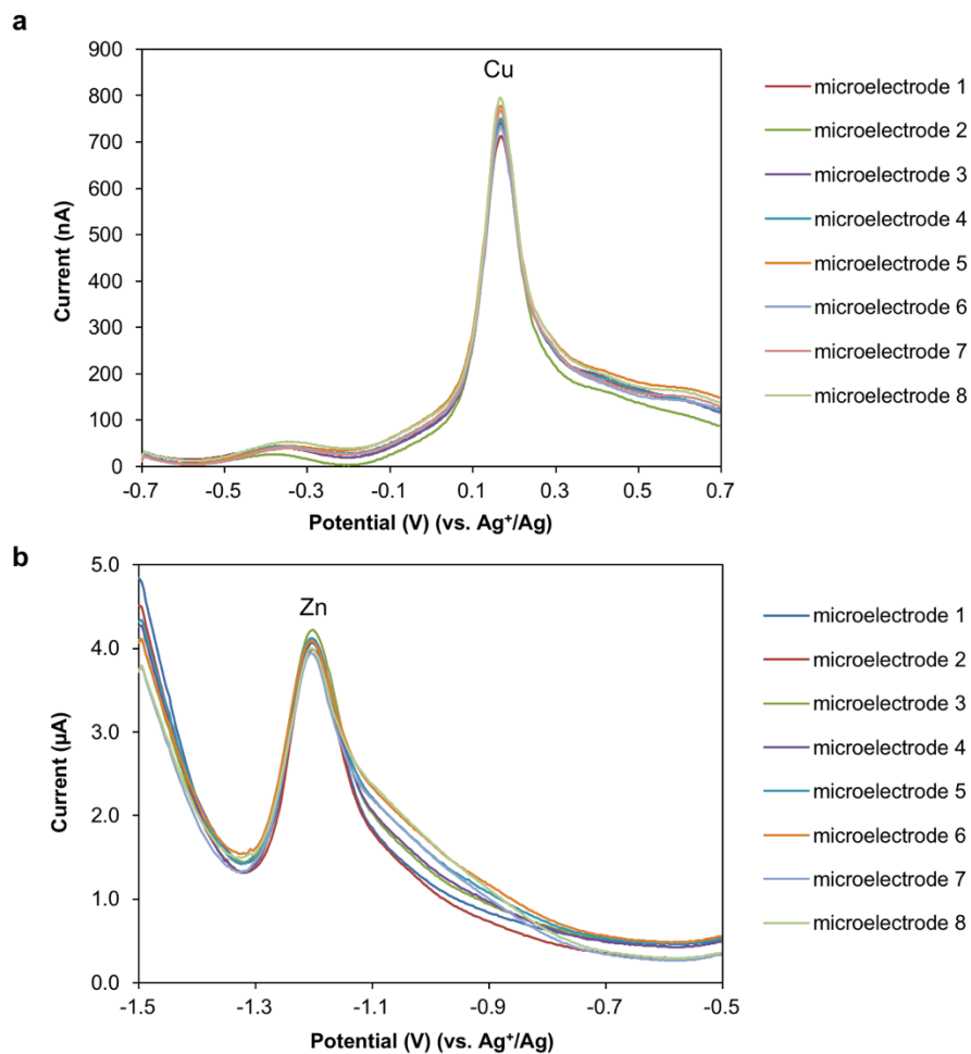
Figure S2. Reproducibility of the microsensor arrays. a) Stripping voltammograms continuously recorded with eight gold microelectrodes in 0.01 M acetate buffer (pH 4.6) containing 50 mM NaCl and 300 μg/L Cu. Preconcentration at -0.7 V for 15 s; other stripping conditions, same as Figure 3a. b) Stripping voltammograms continuously recorded with eight Bi microelectrodes in 0.01 M acetate buffer (pH 4.6) containing 50 mM NaCl and 300 μg/L Zn. Stripping conditions, same as Figure 3c.
