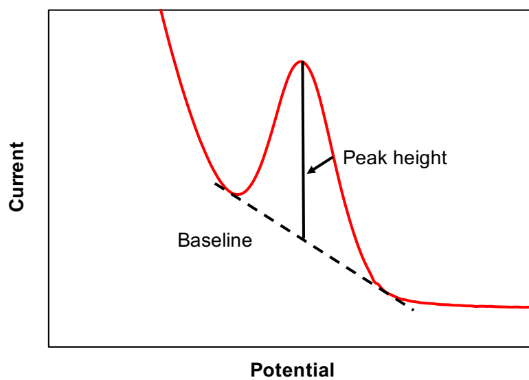
Figure S1. The measurement of peak height from a stripping voltammogram.
