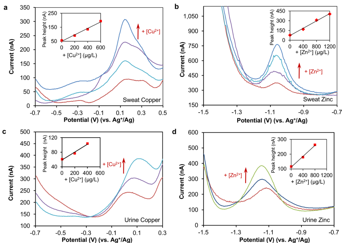
Figure S3. Heavy metal analysis in human body fluids. a, b) Stripping voltammograms for detection of copper (a) and zinc (b) in raw human sweat (collected from a volunteer subject during indoor cycling exercise) and in sweat samples with successive standard additions of Cu and Zn respectively. c, d) Stripping voltammograms for detection of copper (c) and zinc (d) in raw human urine (collected from the same volunteer subject) and in urine samples with successive standard additions of Cu and Zn respectively. The red curves are stripping voltammograms from raw body fluids. Insets in a-d, the corresponding calibration curves for the heavy metal analysis in body fluids.
