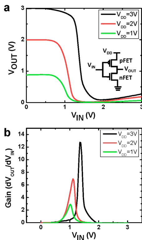
Figure 4. (a) Voltage transfer characteristics of a WSe 2 CMOS inverter at different supply voltages. (b) Direct current voltage gain of the inverter at different V_{\text{DD}} .
